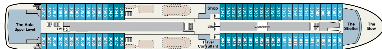
DECK 3
